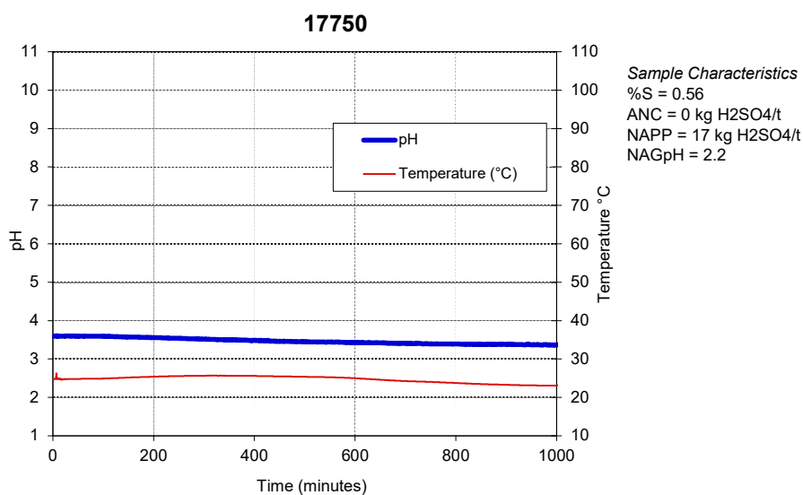
Figure C17: Kinetic NAG graph for Coal.
