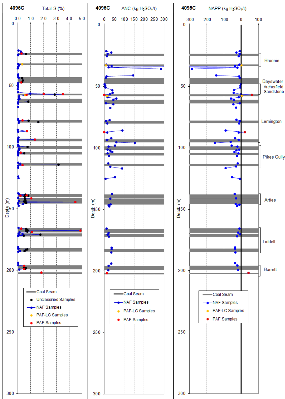
Figure 21: Total S, ANC and NAPP profiles for hole 4095C.
