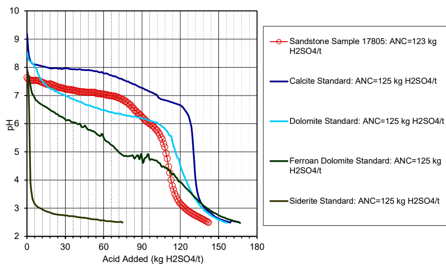
Figure C12: ABCC profile for sample 17805 with an ANC value close to 125 kg H 2 SO 4 /t. Carbonate standard curves are included for reference.
