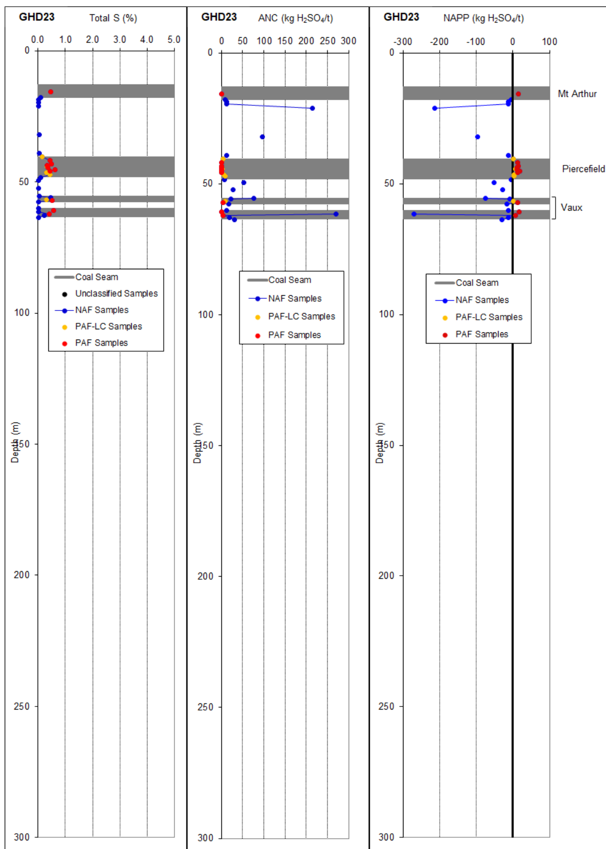
Figure 22: Total S, ANC and NAPP profiles for hole GHD23.
