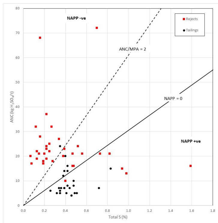
Figure 28: Acid base account (ABA) plot showing ANC versus total S split by rejects and tailings samples.
