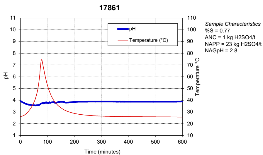
Figure C20: Kinetic NAG graph for Siltstone.
