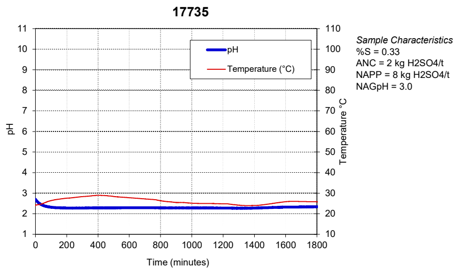
Figure C15: Kinetic NAG graph for Siltstone.
