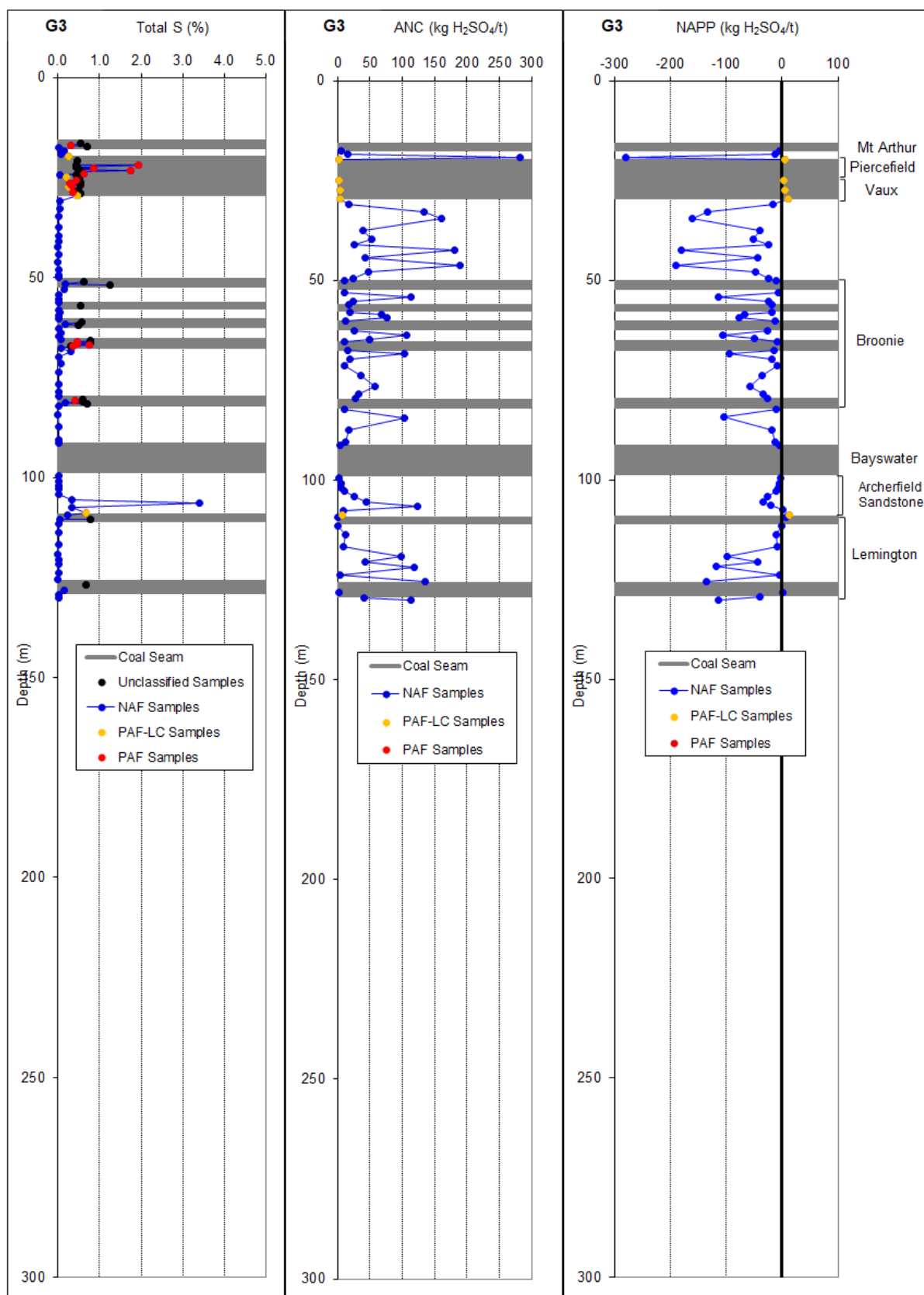
Figure 20: Total S, ANC and NAPP profiles for hole G3.
