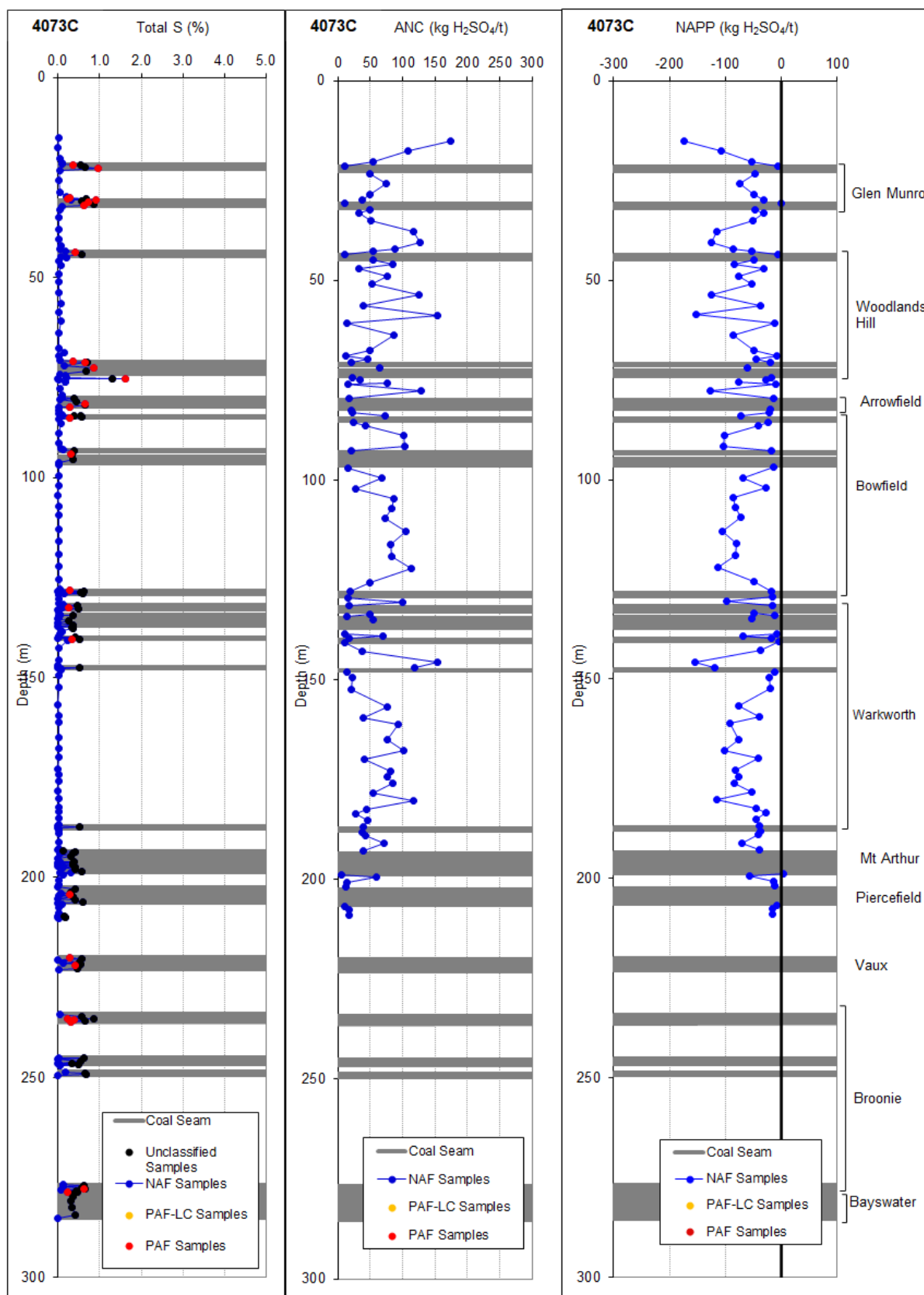
Figure 23: Total S, ANC and NAPP profiles for hole 4073C.
