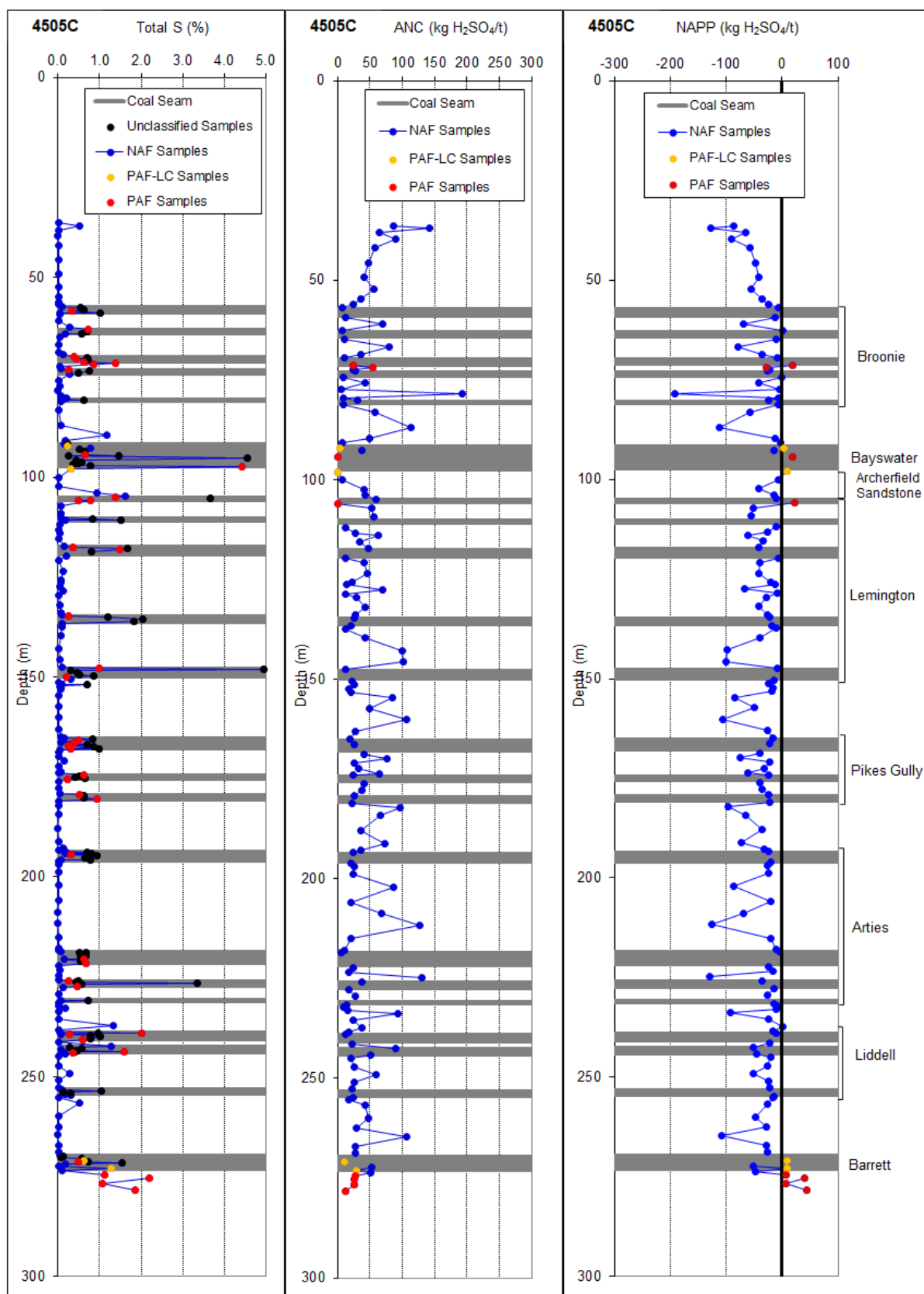
Figure 19: Total S, ANC and NAPP profiles for hole 4505C.
