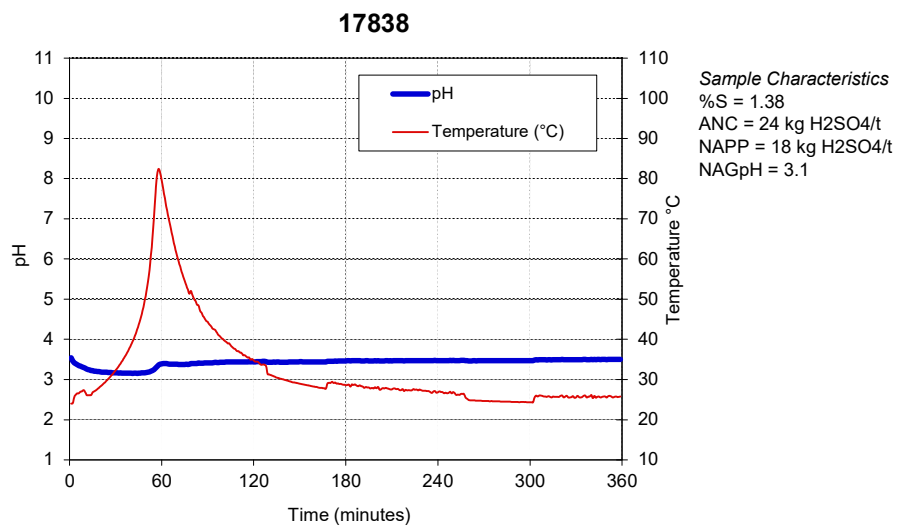
Figure C18: Kinetic NAG graph for Siltstone.
