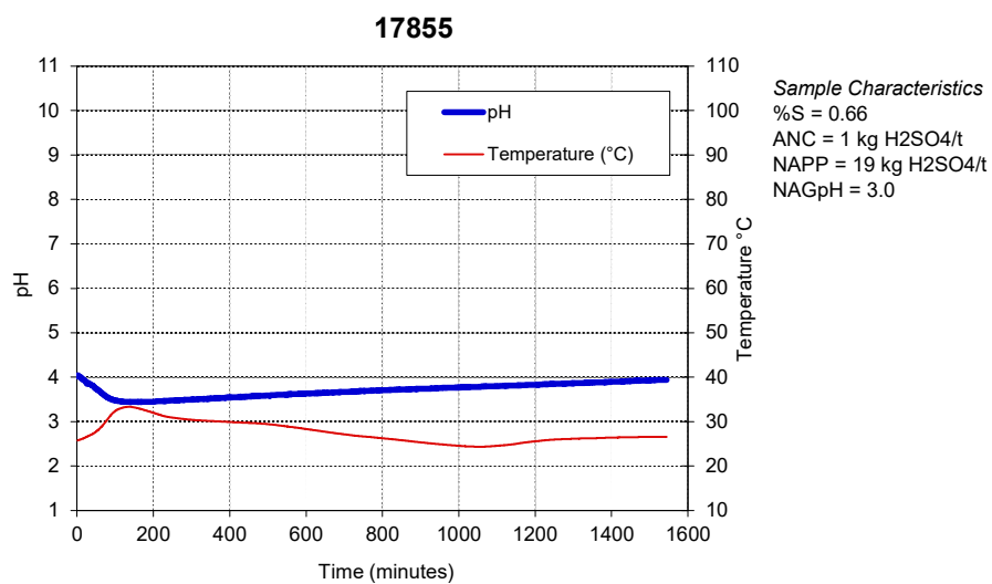
Figure C19: Kinetic NAG graph for Coal.
