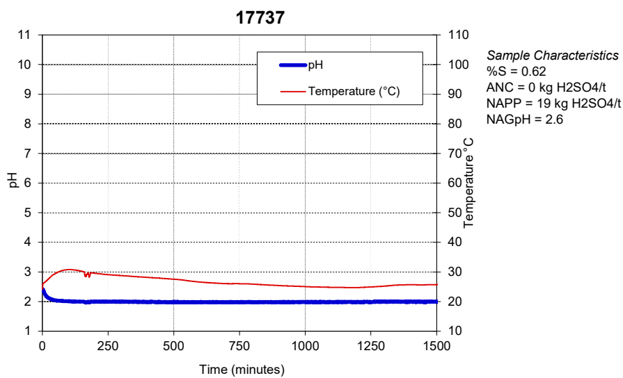
Figure C16: Kinetic NAG graph for Mudstone.
