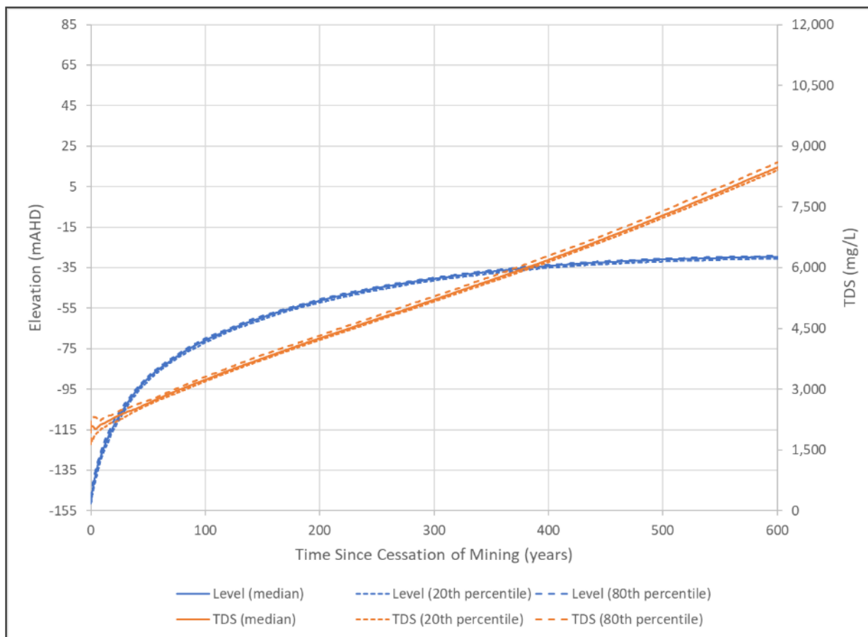
Figure 6.4 HVO South pit lake recovery and salinity (Engeny 2026a)
