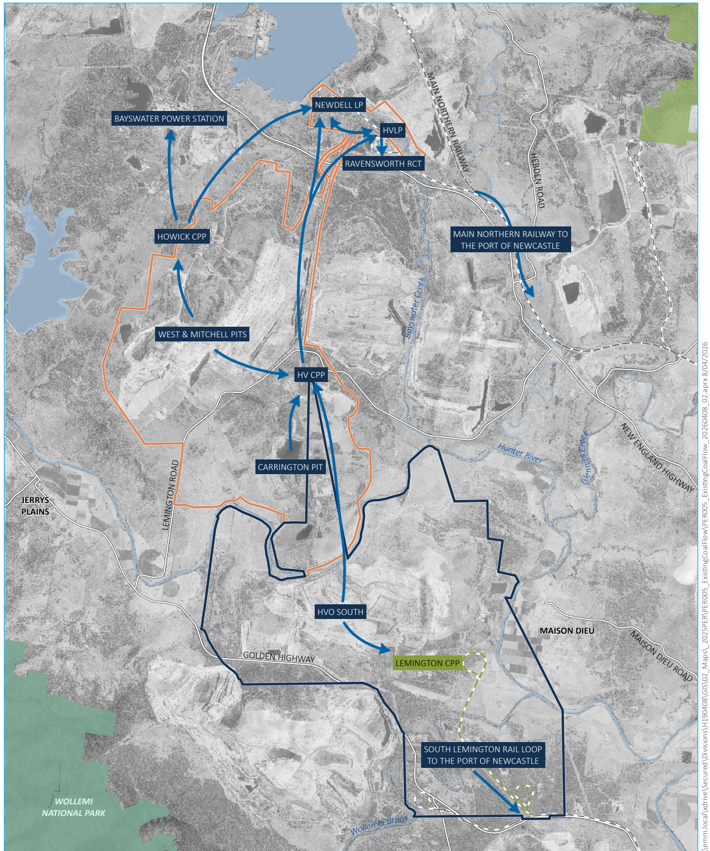
HVO Complex existing coal flow diagram
