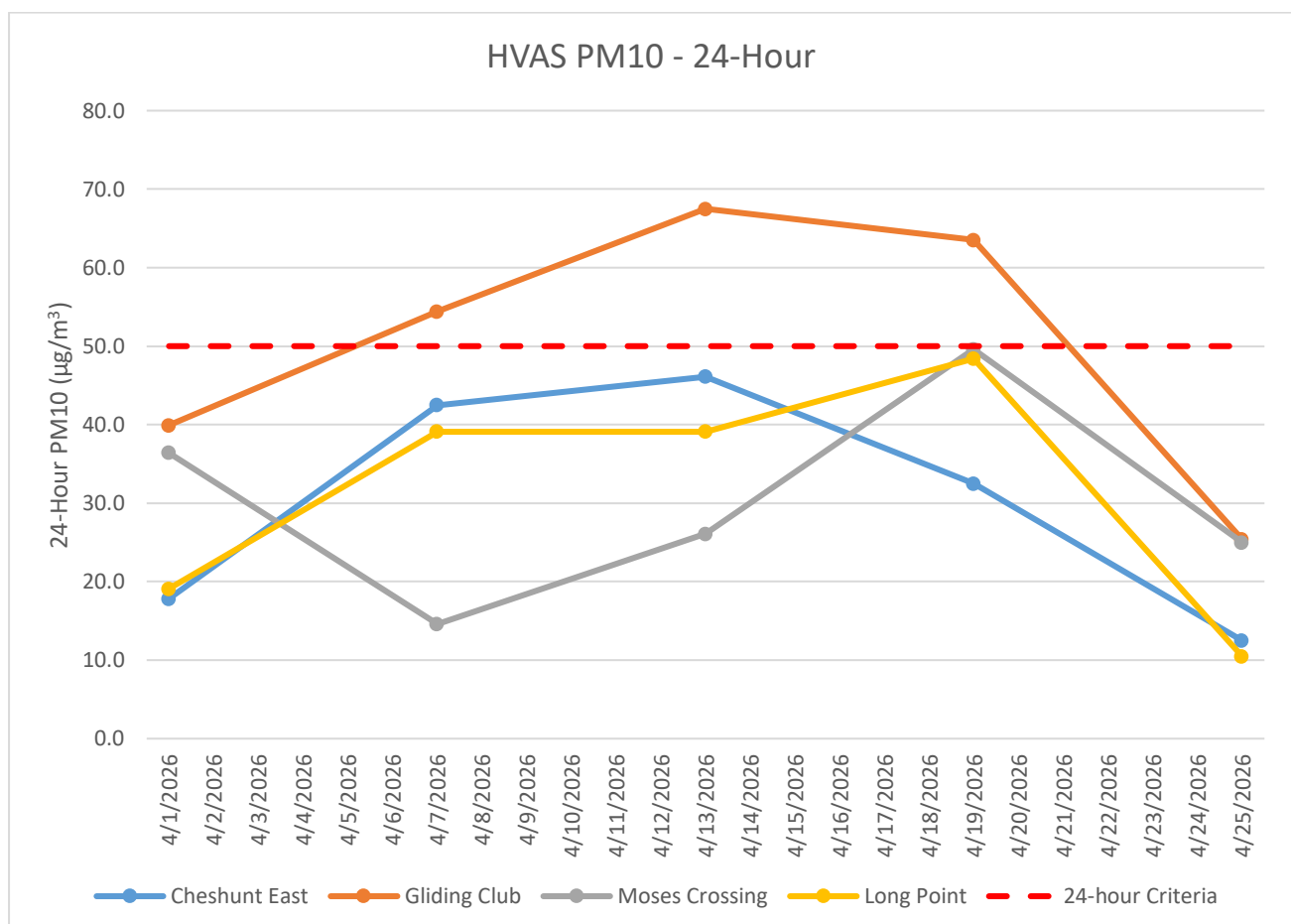
Figure 6 – Individual \text{PM}_{10} Results for the Reporting Period
