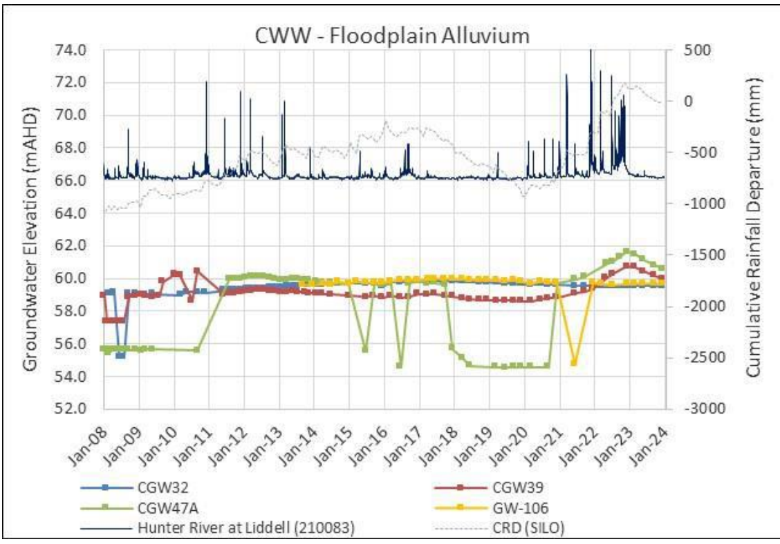
Figure 3. Groundwater levels at Carrington West Wing-Floodplain Alluvium
