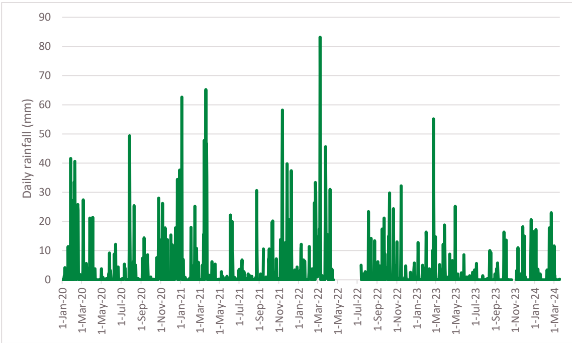
Figure 5. Daily Rainfall data from 1 January 2020 to 18 March 2024 (Singleton Defence AWS 061430).
