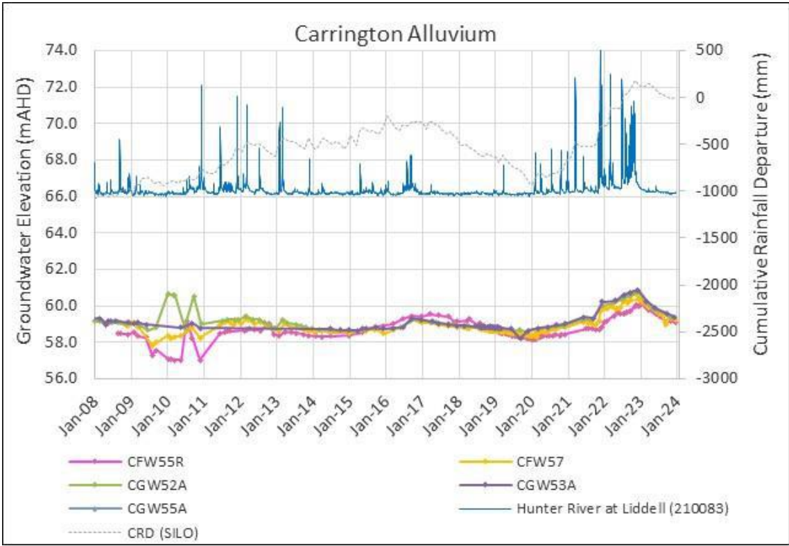
Figure 4. Groundwater levels at Carrington Alluvium
