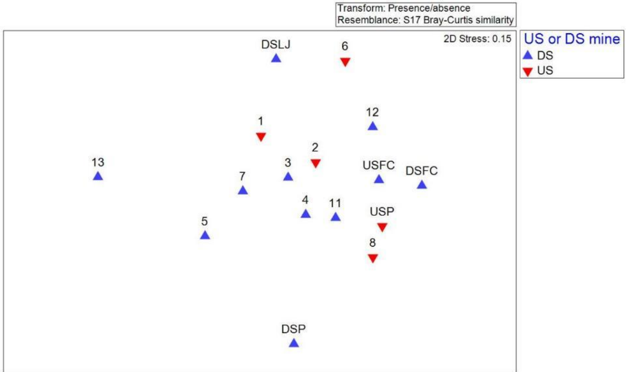
Figure 17: nMDS plot of macroinvertebrate communities at control (red triangle) and impact (blue triangle) sites during January 2022
