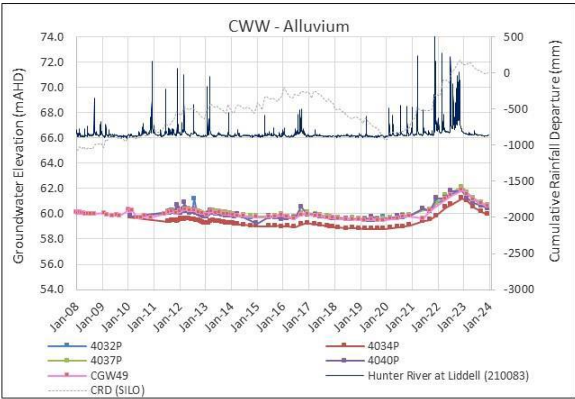
Figure 2. Groundwater levels in Carrington West Wing Alluvium (Umwelt 2024)
